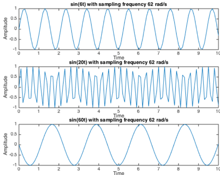
Figure C.6: Aliasing example
