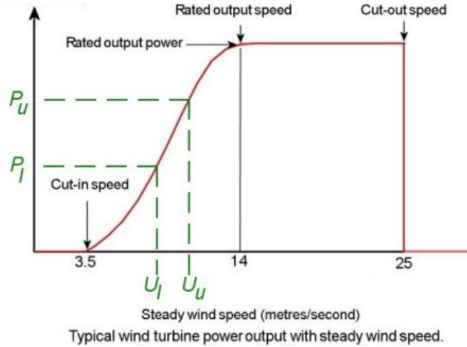
Figure 1: Wind turbine power profile 1
