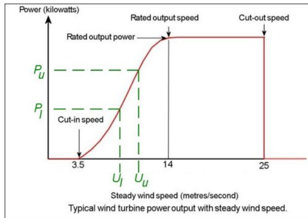
Figure 1: Wind turbine power profile 1
