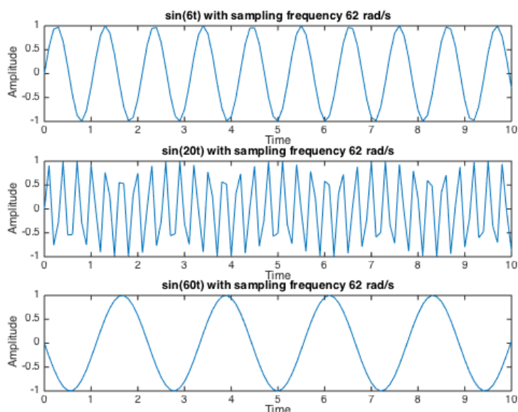
Figure 8.6: Aliasing example
