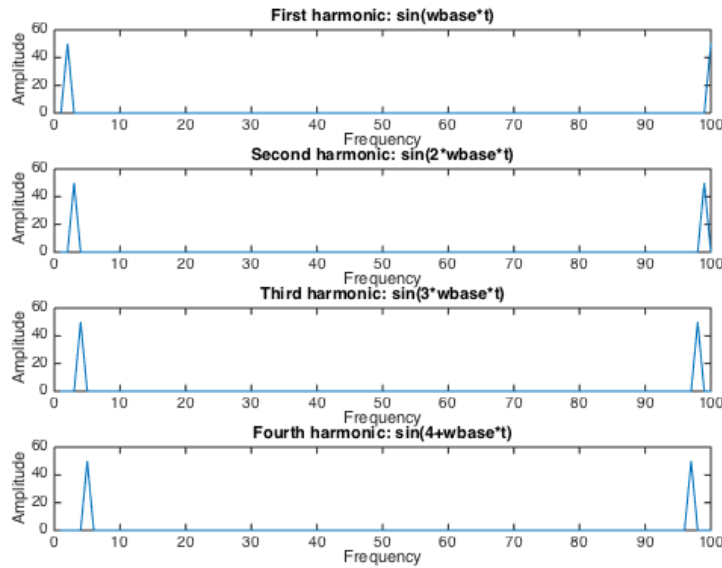
Figure 8.9: Base frequency, second, third and fourth harmonic in frequency domain
