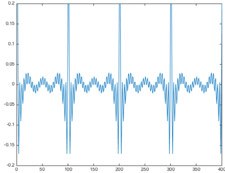
Figure 8.11: Multisine with positive interference clipped at the entrance
