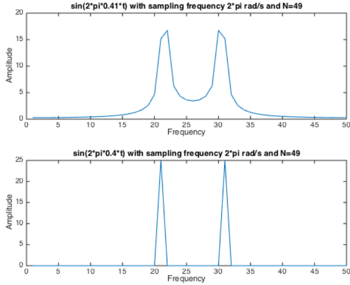
Figure 8.7: The first graph shows leakage, and the second ones does not
