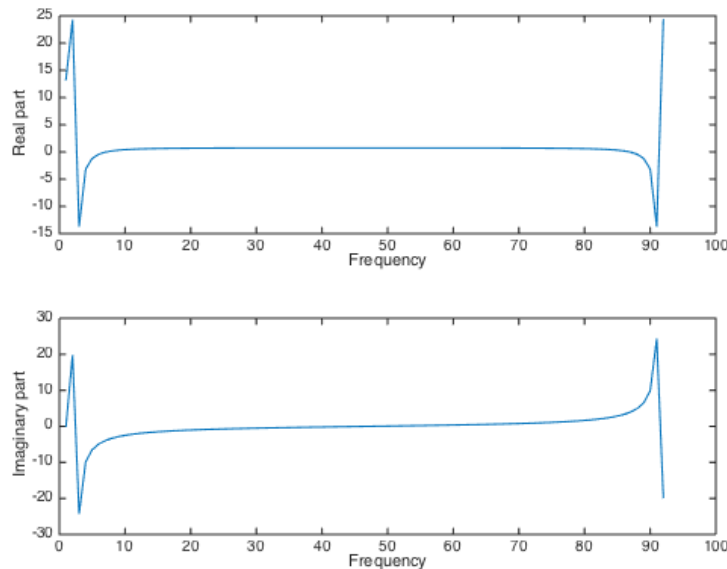
Figure 8.5: DFT example to visualise DFT property
