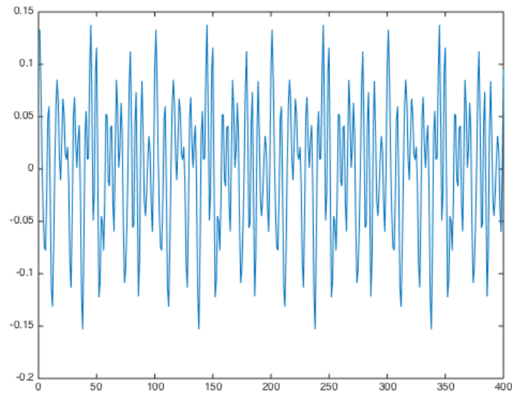
Figure 8.12: Multisine without positive interference, specially designed
