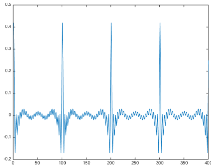
Figure 8.10: Multisine with positive interference
